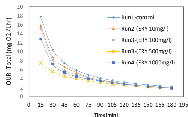
Figure 4. OUR profile for total microorganisms.
